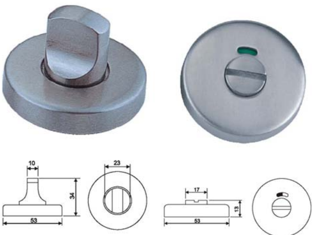
Door Indicator/ REF:: 901001
