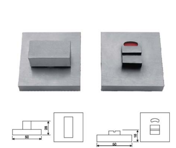
Door Indicator/ REF:: 901008
