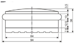
Door Stopper/ REF:: 500075
