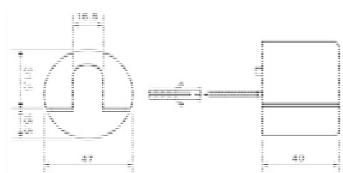
Door Stopper/ REF:: 500078
