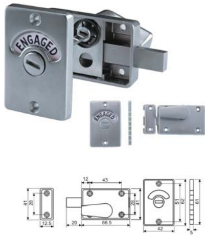
Door Indicator/ REF:: 901000
