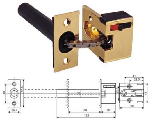
Door Guard/ REF:: 520040
