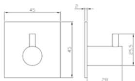
Clothes Hook/ REF:: 621105
