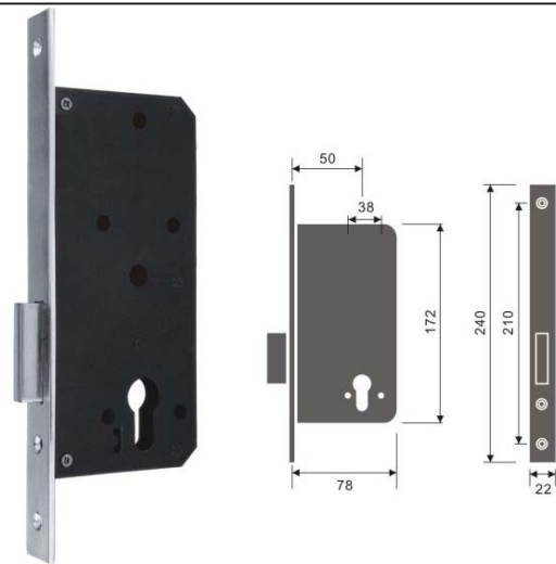
Mortise Door Lock/ REF:: 700004
