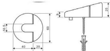
Door Stopper/ REF:: 500076
