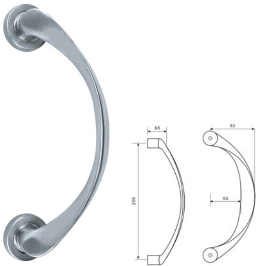
Casting Pull Handle/ REF:: 480001
