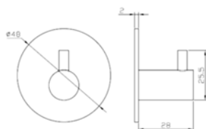
Clothes Hook/ REF:: 621101
