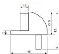
Door Stopper/ REF:: 500003
