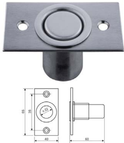
Dust Proof Socket/ REF:: 530005
