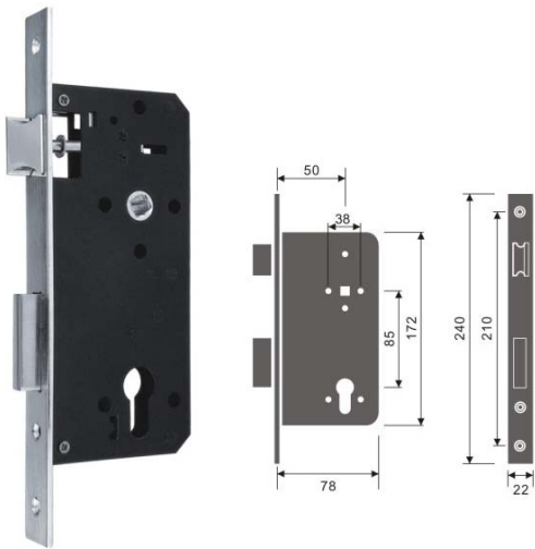
Mortise Door Lock/ REF:: 700001
