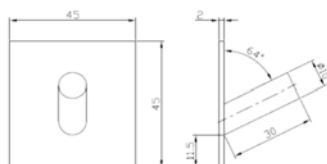
Clothes Hook/ REF:: 621092
