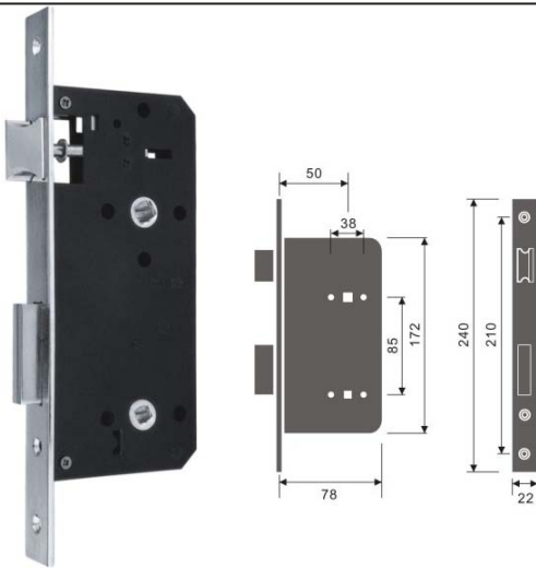
Mortise Door Lock/ REF:: 700003
