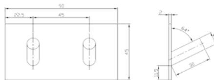
Clothes Hook/ REF:: 621093
