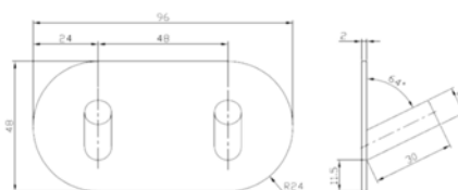
Clothes Hook/ REF:: 621091
