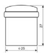
Door Stopper/ REF:: 500063
