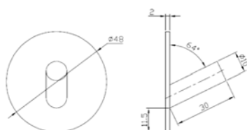
Clothes Hook/ REF:: 621090
