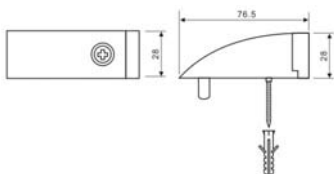
Door Stopper/ REF:: 500077
