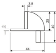
Door Stopper/ REF:: 500001
