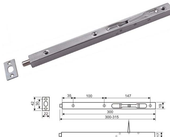
Door Bolt/ REF:: 510004
