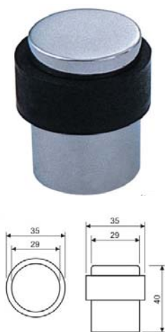
Door Stopper/ REF:: 500005
