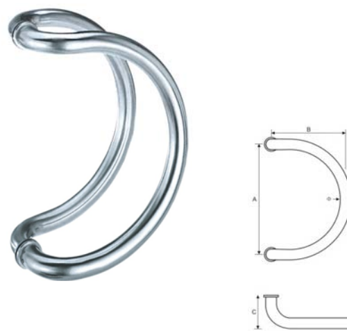
Pull Handle/ REF:: 400216 & 420216
