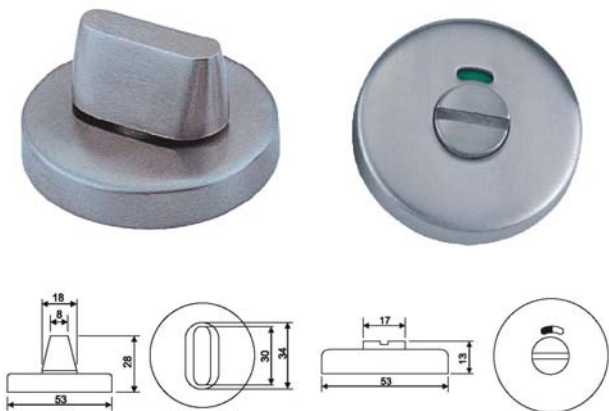
Door Indicator/ REF:: 901005
