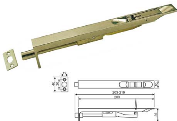
Door Bolt/ REF:: 510006
