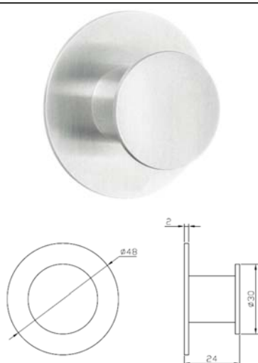
Clothes Hook/ REF:: 621111
