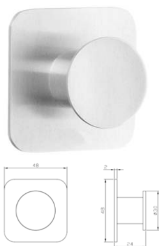
Clothes Hook/ REF:: 621115
