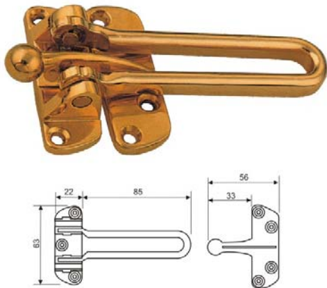
Door Guard/ REF:: 520010
