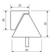
Door Stopper/ REF:: 500010
