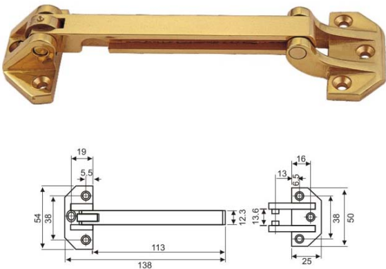
Door Guard/ REF:: 520030
