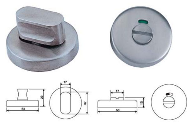
Door Indicator/ REF:: 901006
