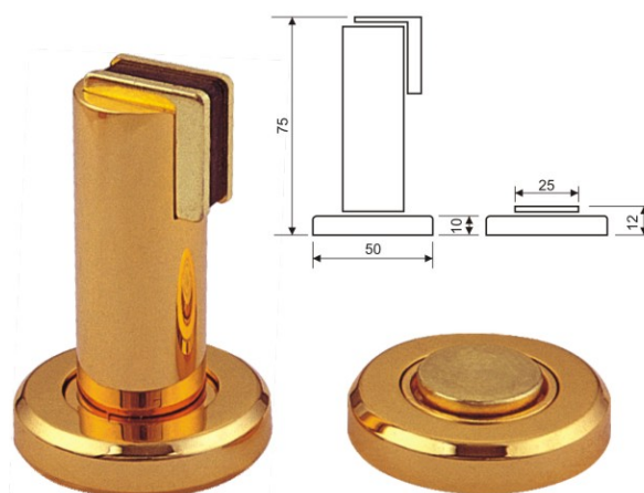
Magnetic Door Stopper/ REF:: 501009
