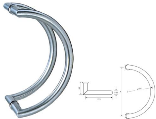
Pull Handle/ REF:: 400211 & 420211
