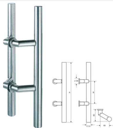
Pull Handle/ REF:: 400206 & 420206
