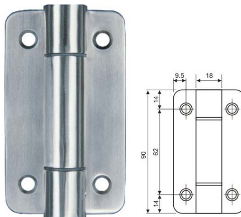
Bathroom Hinge (Without Spring) / REF:: 109302
