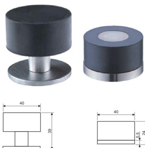
Door Stopper/ REF:: 500008
